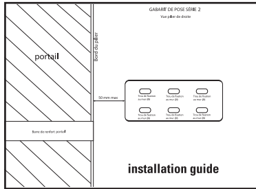
fixing brackets
